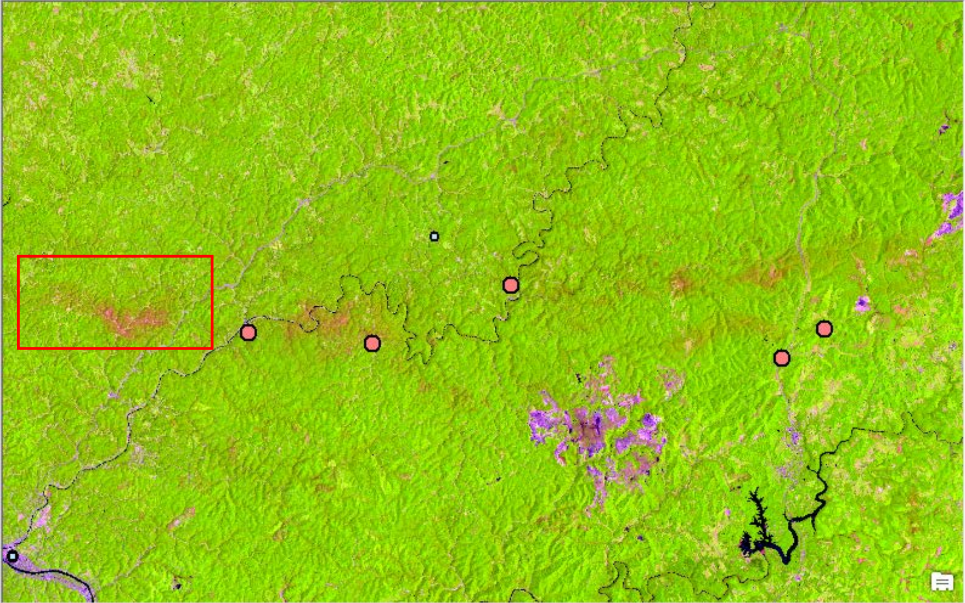
Landsat 5, 543, 07/17/2008
